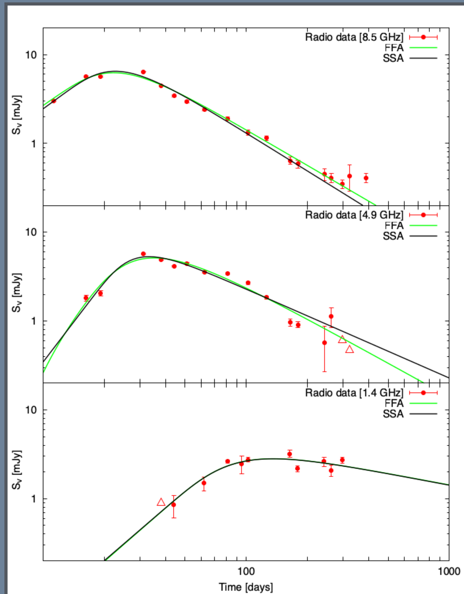
Fig. 1. Radio light curves of SN2004gq at 8.5 GHz (top panel), at 4.9 GHz (middle panel) and at 1.4 GHz (bottom panel).
