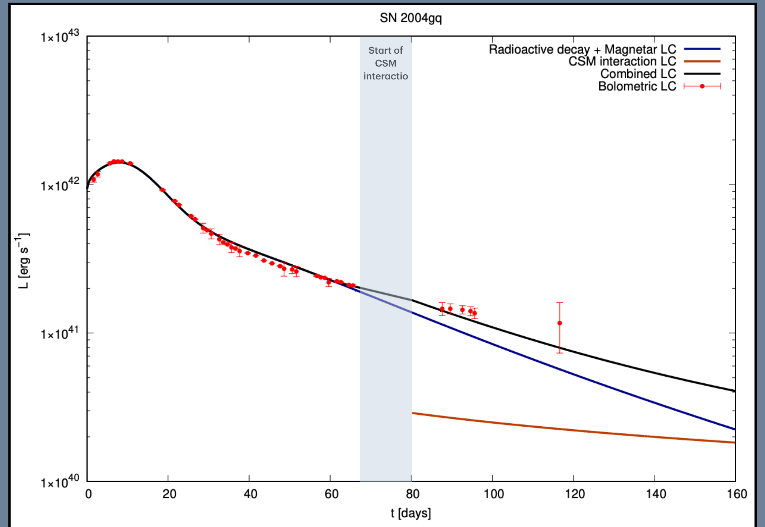
Fig. 2. Comparison of the quasi-bolometric light curve of SN2004gq (red dots) with best-fit model data. The orange and blue curves represent the contribution of the CSM interaction and the photon-diffusion model, respectively, while the black lines show the combined LCs.
